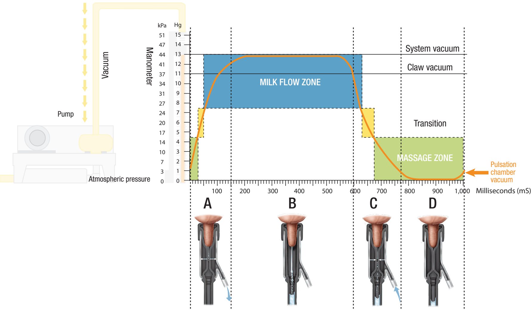
FIGURE 1 The four phases of the pulsation cycle make up liner open and close times for optimal milk harvest
